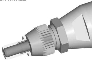
Flush rod on the end of the RIVKLE®
