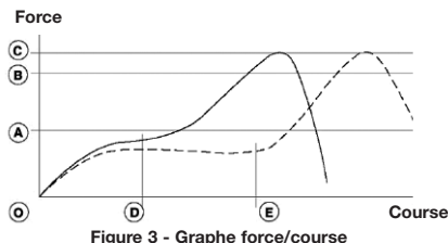
Figure 3 - Graphe force/course
