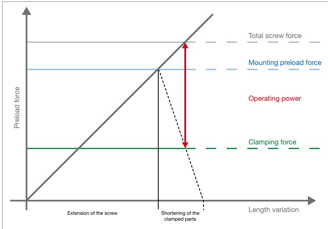
Figure 2.4 Stress diagram
