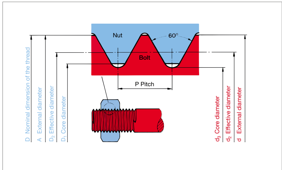
Figure 6.1 Thread profile without clearance
