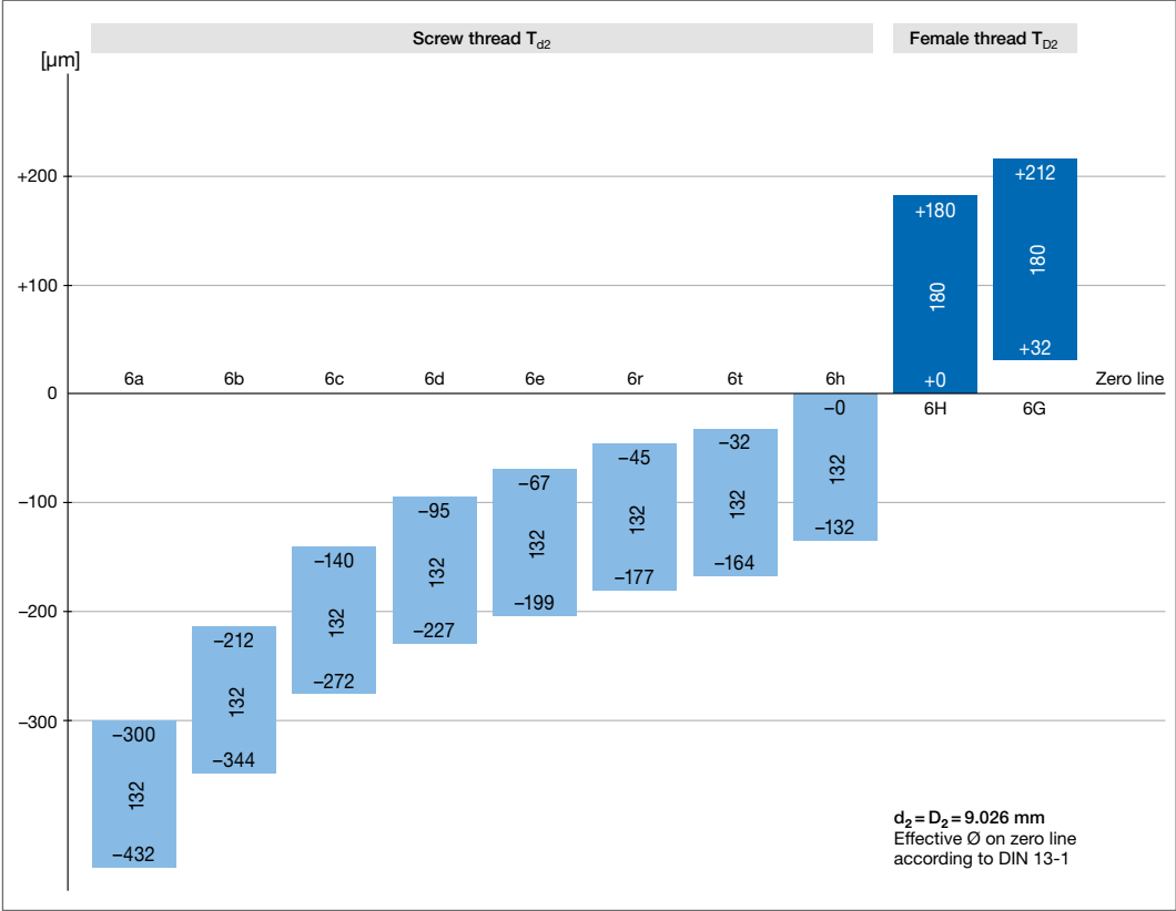
Figure 6.3 Tolerances T d2 and T D2 for the effective diameter d 2 (screw) and D 2 (nut) of an M10 × 1.5 thread.
