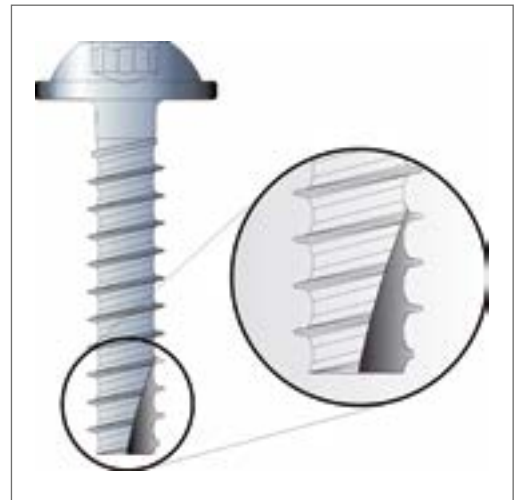
Figure 8.15 Delta PT screw with cutting edge for direct screw connections in thermosetting plastics
