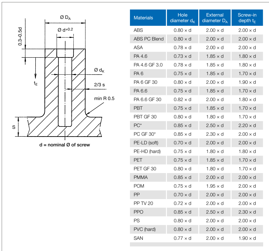
Figure 8.13 Recommended tube design for direct screw fastening with AMTEC® screws
