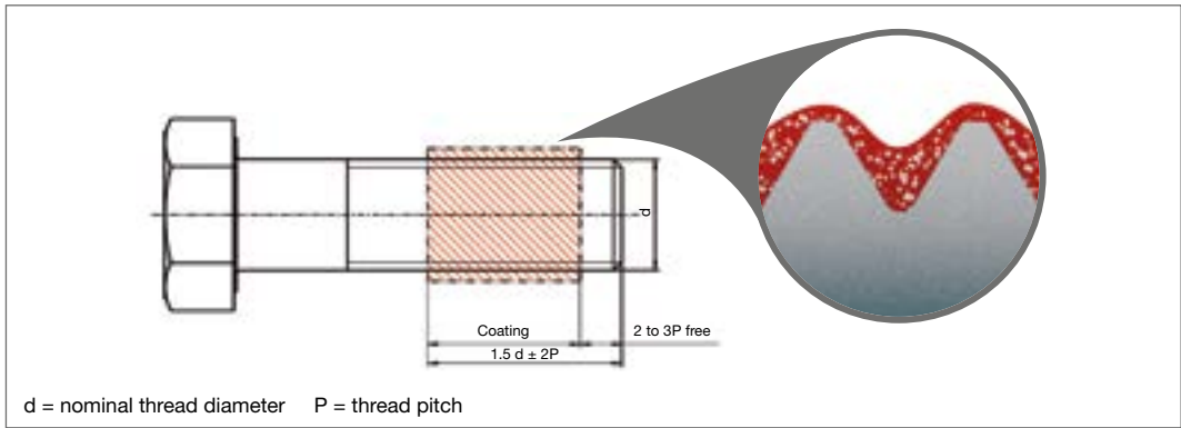
Figure 9.10 Position of coating, e.g. for a hexagon head screw
