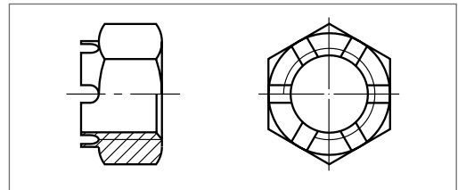
Figure 9.3 Castle nut
