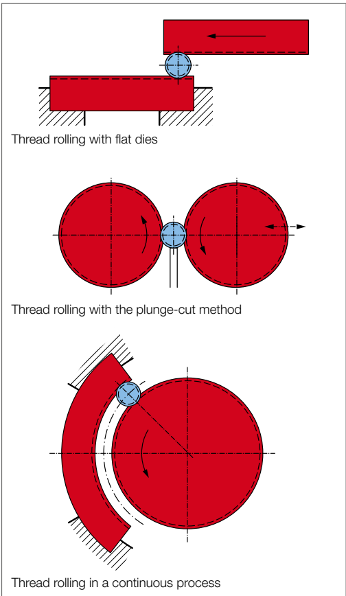
Figure 5.8 The thread production process
