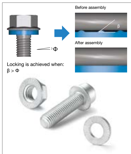
Figure 9.5 Fasteners with ribbings on the bearing surface
