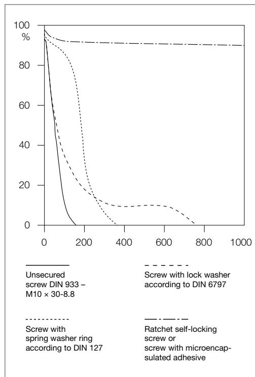
Figure 9.12 Loosening curves of various screw connections subject to dynamic transverse loading
