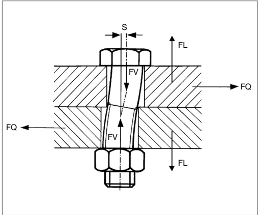
Figure 2.5 Independent loosening and shifting of limit S
