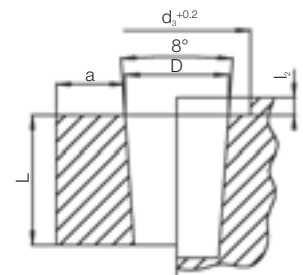
Mounting hole
