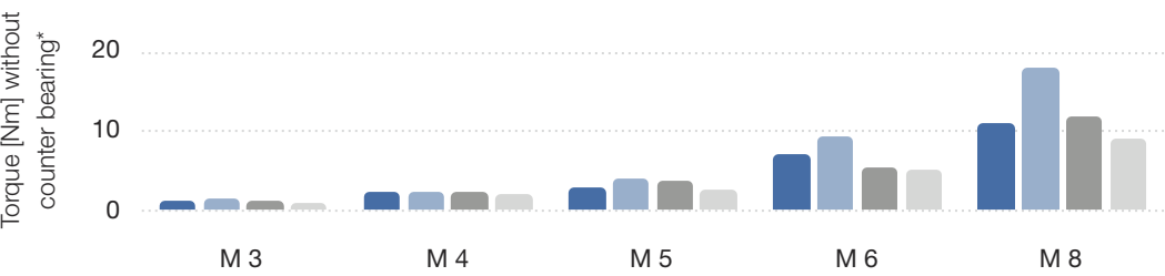
Torque values for HITSERT® M 3 to M 8 tested in different materials
